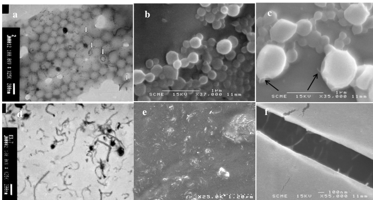
Fig.2. Nanocomposite particles (top) and composite film after annealing (bottom) as observed by TEM (a, d) and SEM (b, c, e, f). Arrow in (a) shows individual CNT entrapped into polymer particles, whereas (b) and (c) shows the non-spherical shapes of the objects due to CNT protruding (showed by black arrows). After annealing, films were composed of long individual nanotubes, visible in the core of the material by TEM (d) or at the surface of the film by SEM (e). A fracture of the film breaks in some extent the CNTs (f). Scales are given vertically and horizontally in TEM and SEM photos.
