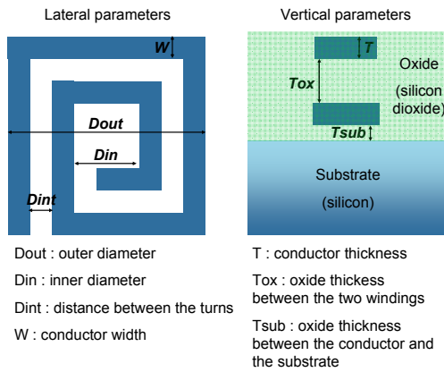
Figure 2: Geometrical parameters of the integrated transformer
