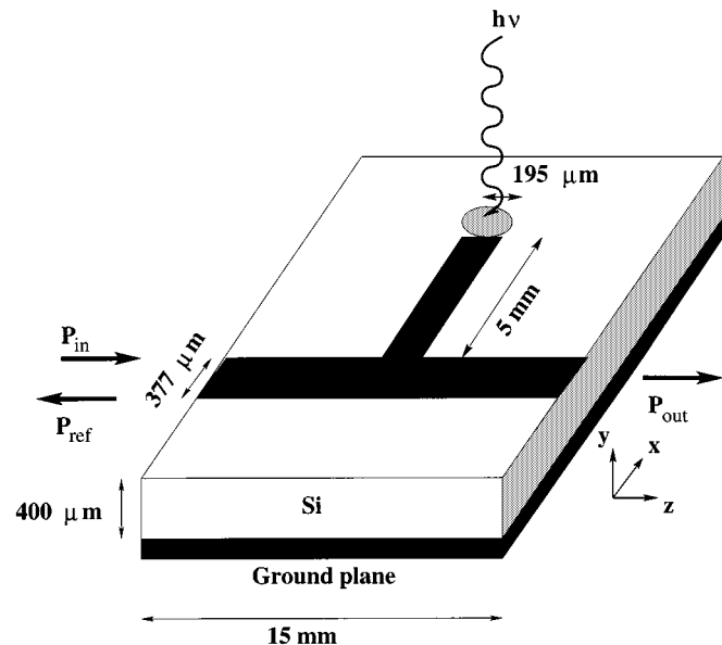
Fig. 1. Physical characteristics of the microstrip line 50 \Omega .
