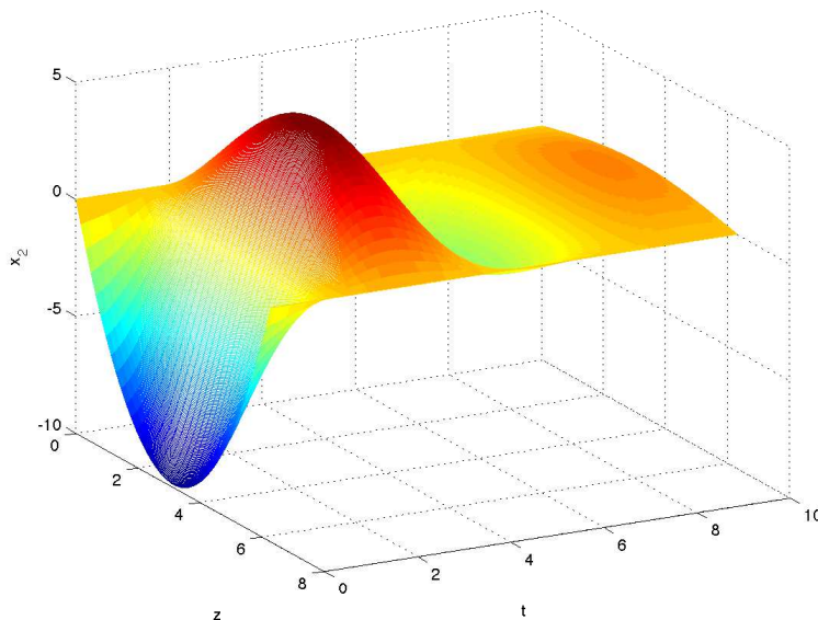
FIGURE 2. Component x_2 of the solution of (52) for t \in [0, 10]
