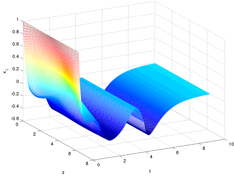
FIGURE 4. Component x_2 of the solution of (53) for t \in [0, 10]
