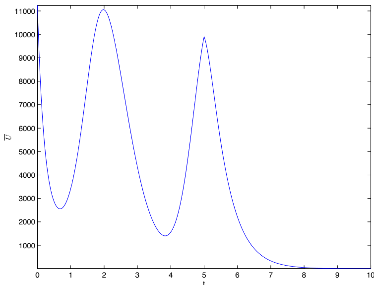
FIGURE 5. Time-evolution of the function \bar{U} given by (54)
