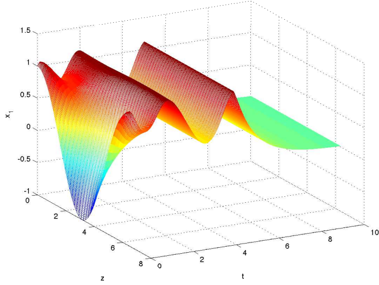
FIGURE 3. Component x_1 of the solution of (53) for t \in [0, 10]
