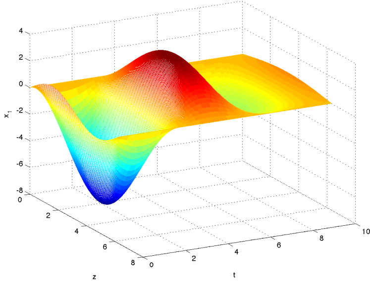
FIGURE 1. Component x_1 of the solution of (52) for t \in [0, 10]
