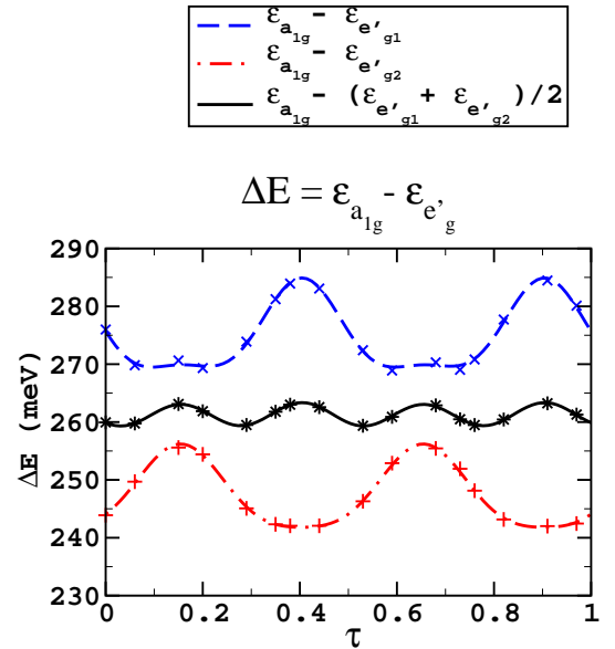
Figure 2. (Color online) 3d cobalt orbital energy splittings: \varepsilon_{a_{1g}} - \varepsilon_{e'_g} , as a function of the incommensurate modulation parameter \tau . Blue curve with crosses: \varepsilon_{a_{1g}} - \varepsilon_{e'_{g1}} splitting, red curve with plus signs: \varepsilon_{a_{1g}} - \varepsilon_{e'_{g2}} splitting, black curve with stars: average \varepsilon_{a_{1g}} - \varepsilon_{e'_g} splitting.
