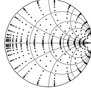
Fig. 10. The complex loads generated by the program.
