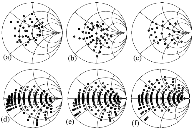
Fig. 22. Measured matched complex loads, under the conditions |S_{11}| < -20 dB and |S_{21}| > -2 dB, at three frequencies: (a) 0.8 GHz (b) 1.0 GHz and (c)
