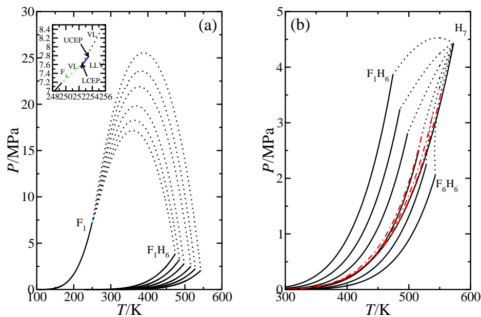
Figure 8. Theoretical predictions of the PT projection of the phase behaviour for the binary mixtures (a) perfluoromethane ( F_1 ) + asymmetric surfactant ( F_XH_6 ) and (b) n -heptane ( H_7 ) + asymmetric surfactant ( F_XH_6 ) using the hetero-SAFT-VR approach. Solid lines describe the vapour-pressure curves of pure components, dotted curves are the gas-liquid critical lines ( (L-V)_1 (black) and (L-V)_2 (green)), dashed line (blue) is the three phase line ( L-L-V ) and dashed-dot line (red) describe the azeotropic line (AZ).
