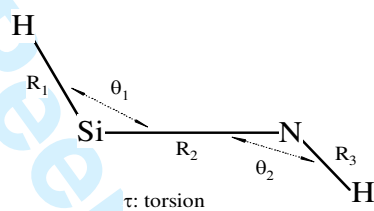
Isomer II
