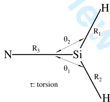
Isomer III
