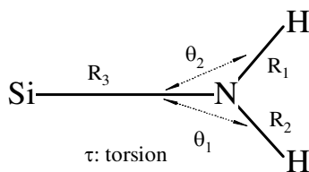
Isomer I
