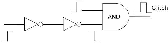
Figure 3. Circuit with glitch formation.
