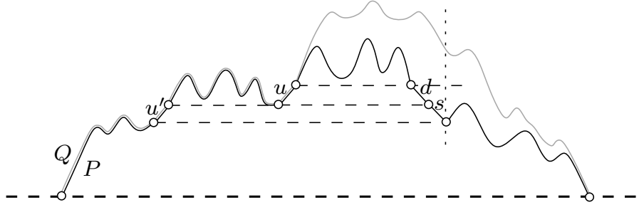
FIGURE 6. Why s cannot be descending.
