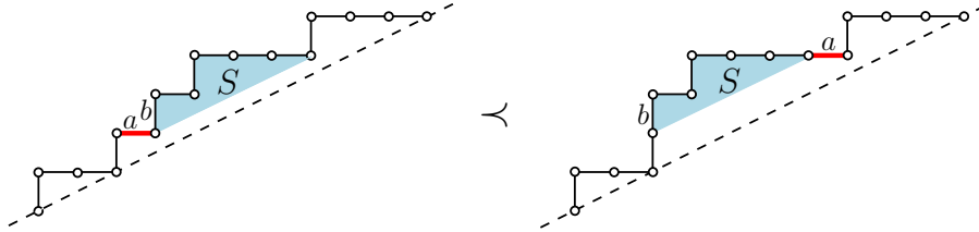
FIGURE 2. The relation < between m -ballot paths ( m = 2 ).
