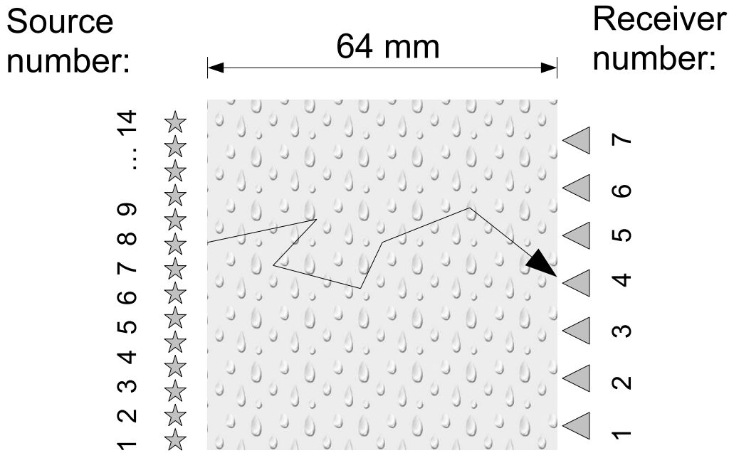
Figure 1. Experimental setup with ultrasound. An air-gel mixture mimics a multiple scattering medium. Coda waves sensed by the receivers (see Fig. 2) are processed like ambient seismic noise : they are autocorrelated and compared from one date to another.
