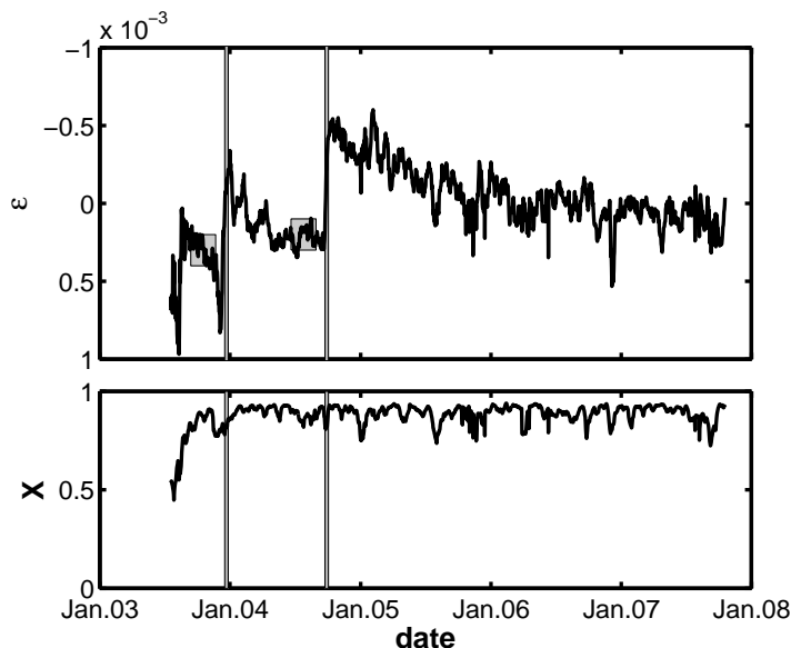
Figure 6. Top: Dilation \epsilon averaged over 78 receiver pairs, using a 5-day sliding window. The grey squares indicate the 70-day reference windows. The best fit \epsilon varied weakly and stochastically over this period, with two notable jumps, after December 22, 2003 and after the Parkfield earthquake on September 28, 2004. The latter jump was followed by a slow recovery. Fluctuations have an rms strength of about 10^{-4} . Bottom: Dilation coefficient X , the maximum value of the dilation coefficient X , averaged over 78 receiver pairs.
