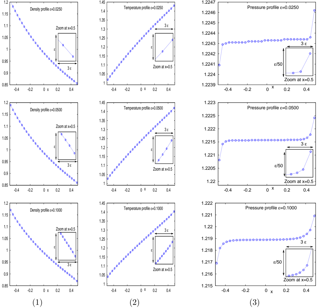
FIGURE 3. Flow generated by a gradient of temperature: (1) density and (2) temperature (3) pressure for various Knudsen numbers \epsilon = 0.025, 0.05 and 0.1 .
