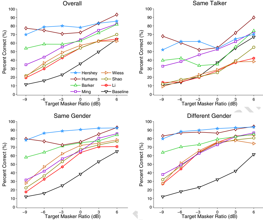
Fig. 3. Recognition results on the two-talker data sets for all systems published in this issue.
