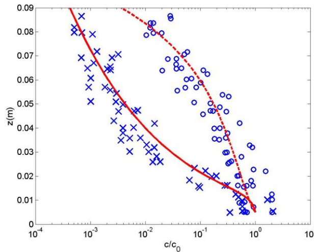
Figure 1: Time-averaged concentration profiles over wave-induced ripples. Symbols: measurements (McFetridge and Nielsen, 1985), (o) fine; (x) coarse; Curves: solutions of Eq. (2) (Absi 2010).
