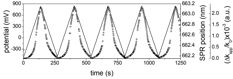
Figure 3. Electrode potential (solid line) and SPR position in wavelength (open circles) versus time. SPR position may also be considered as relative change in SPP wavevector (far right axis).
