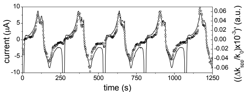
Figure 5. Time dependence of current (solid line) compared with that of the differential of the relative change in SPP wavevector with respect to time (circles).
