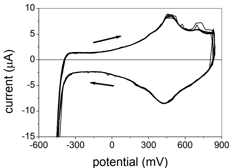
Figure 2. Cyclic voltammogram for a polycrystalline gold-diffraction grating electrode in 0.02M \text{H}_2\text{SO}_4 electrolyte. The potential is cycled between -500 mV and 850 mV at 10 mV/s.
