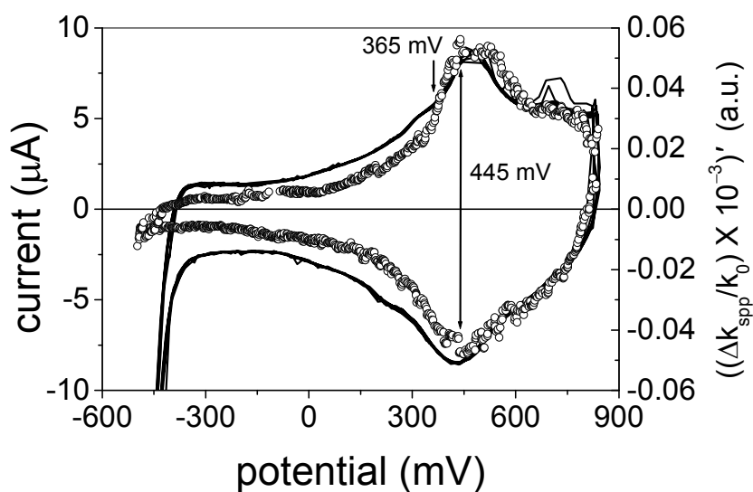
Figure 6. Cyclic voltammogram (solid line), as shown in figure 2, compared with the differential of the relative change in SPP wavevector with respect to time (circles).
