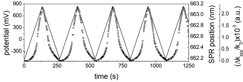
Figure 3. Electrode potential (solid line) and SPR position in wavelength (open circles) versus time. SPR position may also be considered as relative change in SPP wavevector (far right axis).
