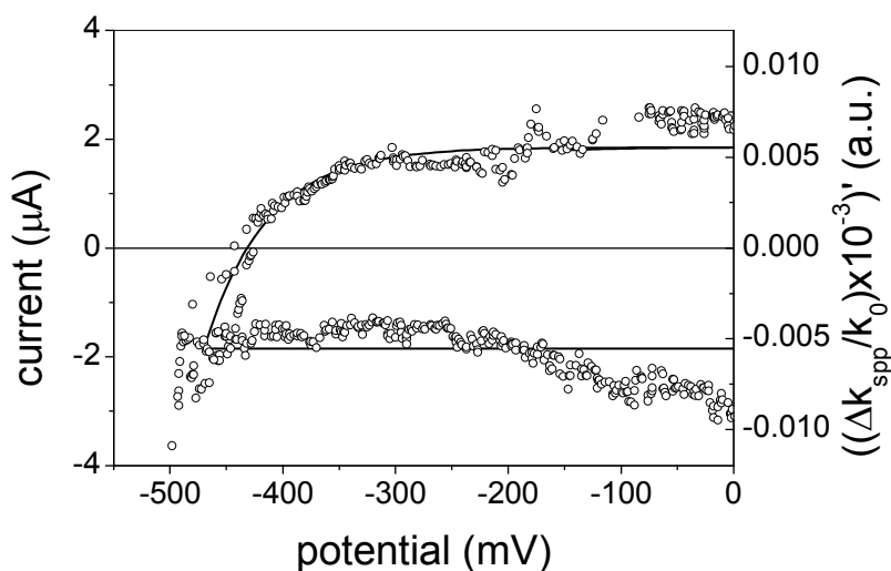
Figure 7. Computer-modelled current-potential response of a capacitor (185 \mu\text{F} ) and resistor (30 \text{k}\Omega ) in series (line). Differential of the relative change in SPP wavevector with respect to time (circles).
