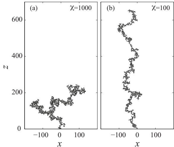
FIG. 3. Air paths from the numerical simulations. Note first that the numerical procedure allows the creation of side branches. For the same injected volume, thus the same number N = 4000 of occupied vertices, one observes that the geometry of the path depends drastically on the control parameter \chi [(a) \chi = 1000 ; (b) \chi = 100 ]. As expected and also observed experimentally, for smaller \chi (larger gravity effects) the finger exhibits less branches and reaches a larger height.
