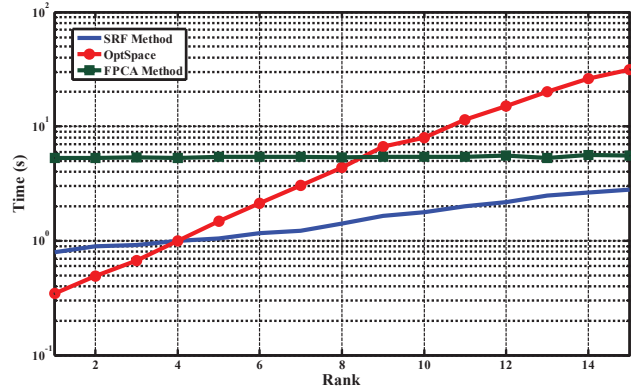
Fig. 1 Execution time vs. rank
