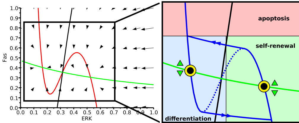
Figure 5: The ‘hysteresis cycle’ scenario. Daughter cells initially inherit half of their mother’s protein level, ‘choose’ one of the stable branches depending on their exposition to Fas-ligand, and then move on these branches which form an hysteresis cycle, making the decision hardly reversible. Shown with yellow circles are the two possible positions for newborn cells exposed to exactly the same value of Fas-ligand on the hysteresis cycle. One can see how the initial choice is important: cells whose mother had low Fas values will be located on the lower branch, those whose mother had sufficiently high Fas values will switch to the upper branch.
