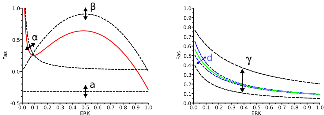
Figure 1: Null-clines f and g defined in (3) and (4). Left panel: the f null-cline (solid red line) and the impact of parameters of equation (1). Right panel: the g null-cline (solid green line) and the impact of parameters of equation (2).
