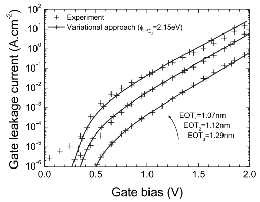
FIG. 9. Experimental and simulated gate current densities vs gate bias for different \text{SiO}_2\text{-HfO}_2 gate stacks. (See the text for details). Data can be fitted using the variational approach with \phi_{\text{HfO}_2} = 2.15 eV barrier.
