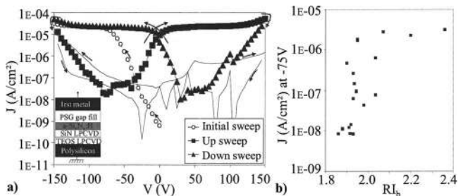
FIG. 3. (a) J\text{-}V on PMD stack. Curve with symbols refers to the worst a\text{-Si}_x\text{N}_y\text{:H} data retention case ( RI_i=2.507 and RI_b=1.95 ). Curve without symbol refers to the best a\text{-Si}_x\text{N}_y\text{:H} data retention case ( RI_i=1.88 and RI_b=1.86 ) and (b) leakage current measured at -75 V on the initial I\text{-}V sweep according to RI_b .
