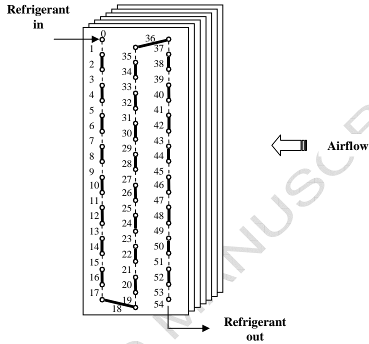
Fig. 2. Tested gas cooler (Coil A) with numbered pipes
