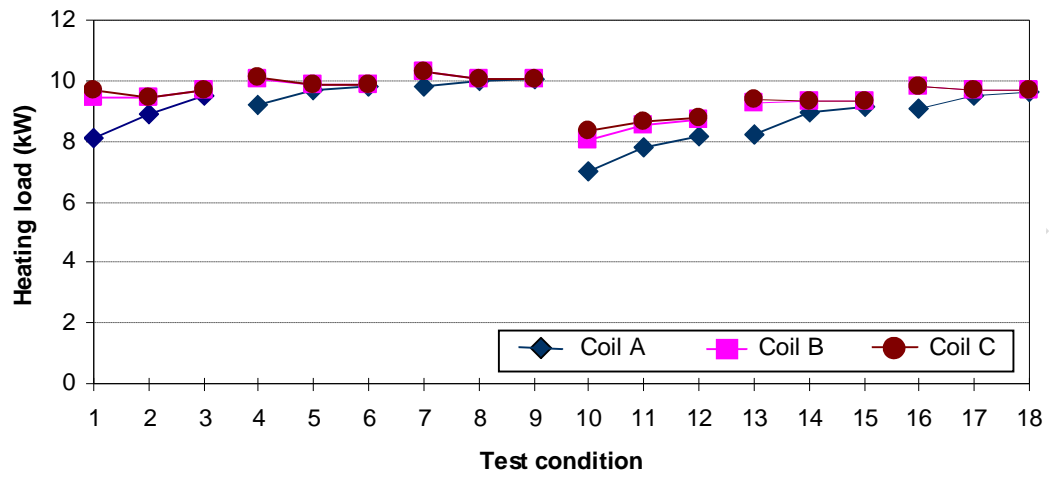
Fig. 11. Simulated heating loads for Coil A, B and C at various test conditions
