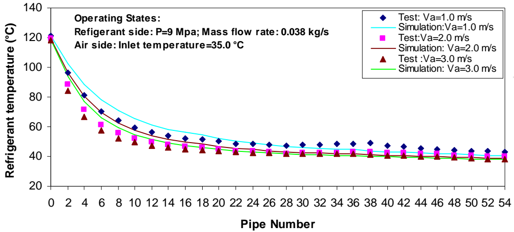
Fig. 4. Comparison of simulation with test results of test condition Nos. 10 to 12 for refrigerant temperature profile.
