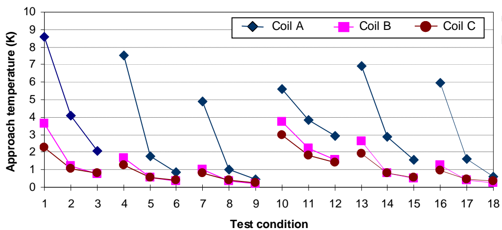
Fig. 9. Simulated approach temperatures for Coil A, B and C at various test conditions
