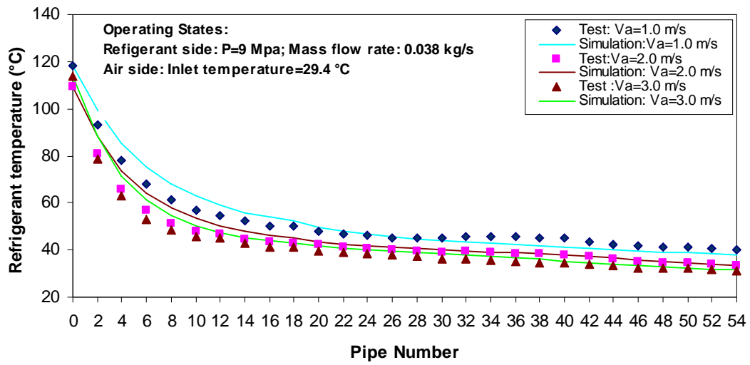
Fig. 3. Comparison of simulation with test results of test condition Nos. 1 to 3 for refrigerant temperature profile.
