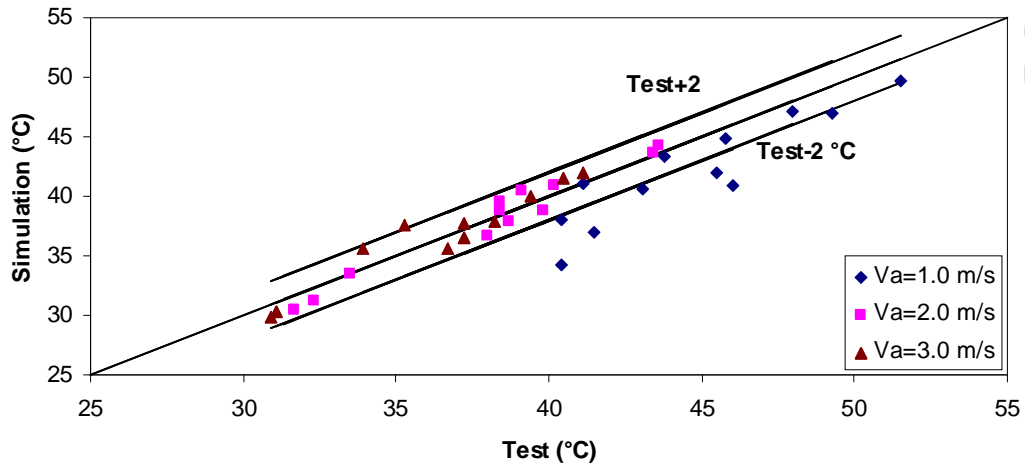
Fig. 7. Comparison of simulation with test results of all test conditions for refrigerant temperatures at gas cooler outlet.
