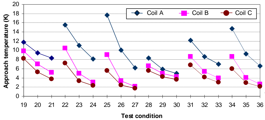
Fig. 10. Simulated approach temperatures for Coil A, B and C at various test conditions (19-36).
