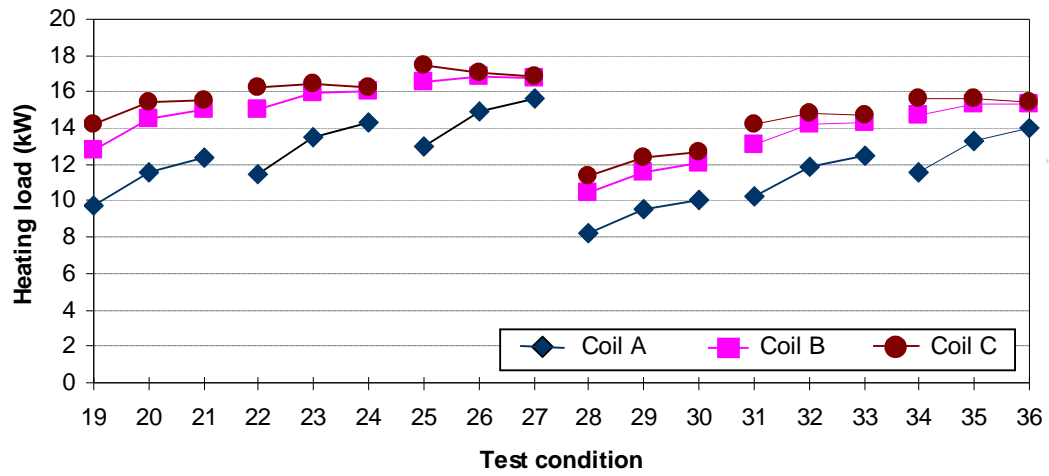
Fig. 12. Simulated heating loads for Coil A, B and C at various test conditions
