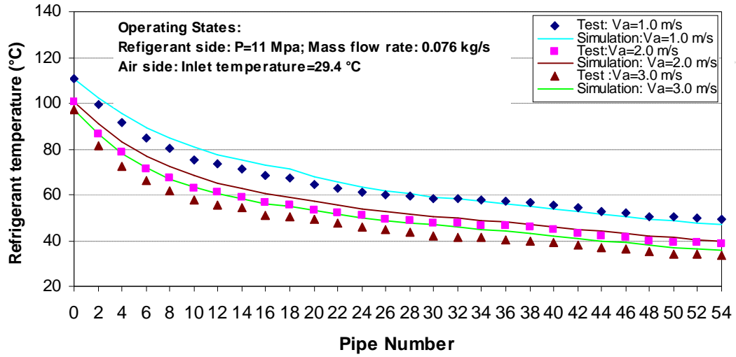
Fig. 6. Comparison of simulation with test results of test condition Nos. 25 to 27 for refrigerant temperature profile.
