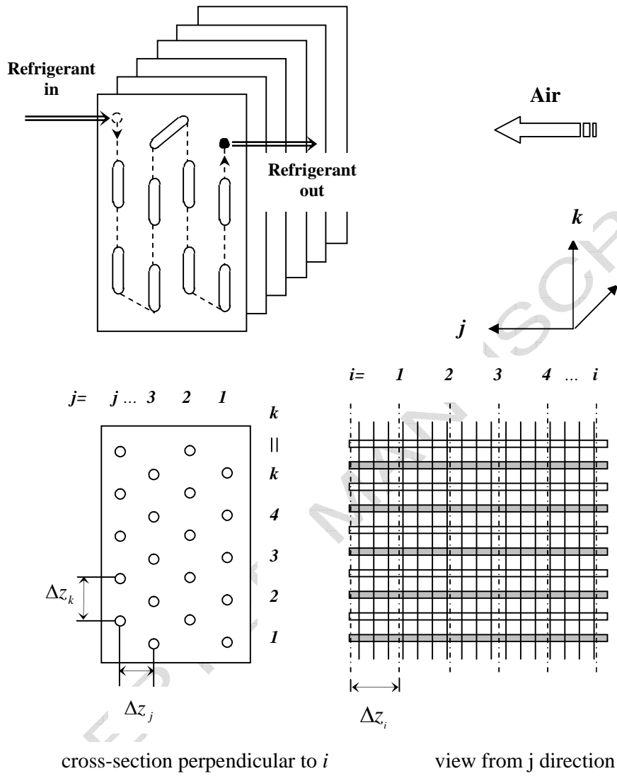
Fig. 1. Three-dimensional coordinate of sub elements in the coil for the gas cooler model
