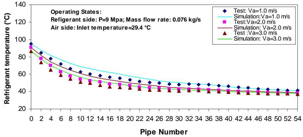
Fig. 5. Comparison of simulation with test results of test condition Nos. 19 to 21 for refrigerant temperature profile.
