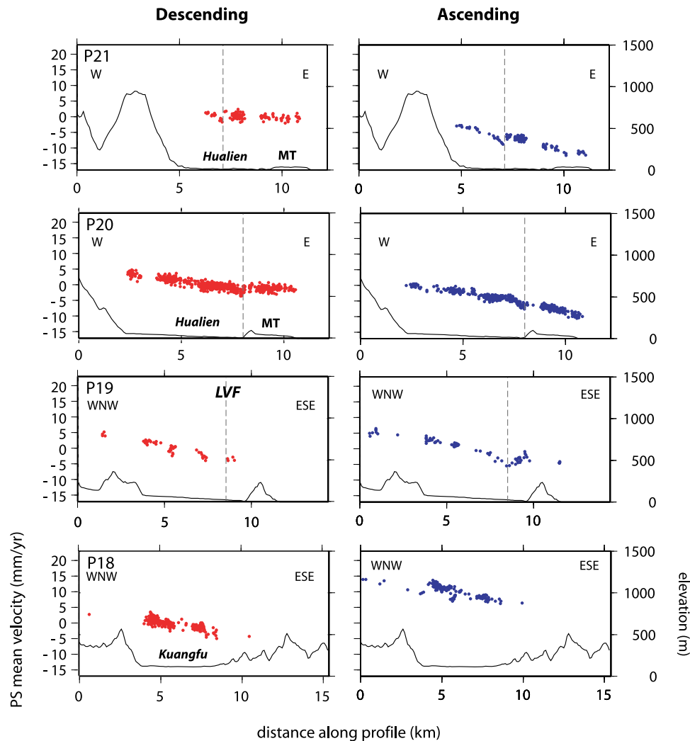
Figure 10. Profiles of PS mean velocities between Ruesuei and the Hualien plain in (left) the descending pass and (right) the ascending pass, superimposed on the topographic profile from the TWD67 40 m resolution digital elevation model. The locations of these profiles are shown in Figure 9. Black dotted lines indicate the location of significant velocity gradient changes in the PS velocity maps. MT, Milun Terraces.
