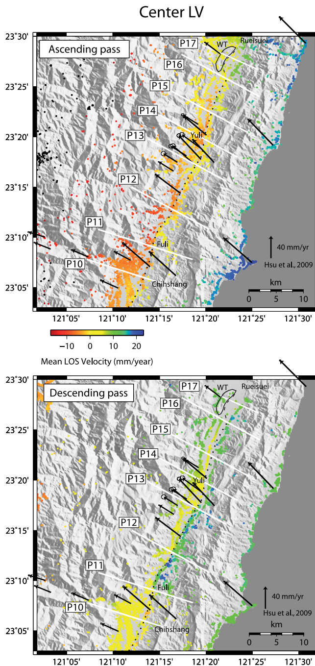
Figure 5. PS mean velocity map in (top) the ascending pass and (bottom) the descending pass between Chihshang and Ruisuei. GPS velocity field is from Hsu et al. [2009b]. Black dotted lines show the location of significant gradient changes in the PS velocity maps. They are all in agreement with the fault traces estimated from geological and geomorphologic field surveys [e.g., Yu et al. , 1997; Shyu et al. , 2006b, 2008]. White lines show the location of the profiles presented in the Figures 6 and 7. WT, Wuhe Tableland.
