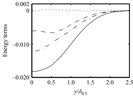
FIGURE 13. Profiles across the self-similar jet averaged over 125r_0 \leq x \leq 145r_0 : \cdots , viscous dissipation; -\cdots- , filtering dissipation; — , total dissipation; \cdots , sum of all the terms in the budget for the turbulent kinetic energy k (curves normalized by \rho_c u_c^3 \delta_{0.5} ).
