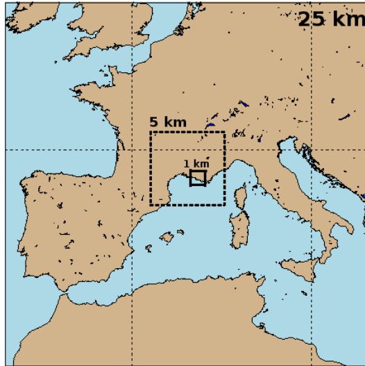
Figure 1: Meso-NH nested domains used in the Lançon-de-Provence case study from the coarse 25-km grid down to the fine 1-km grid.
