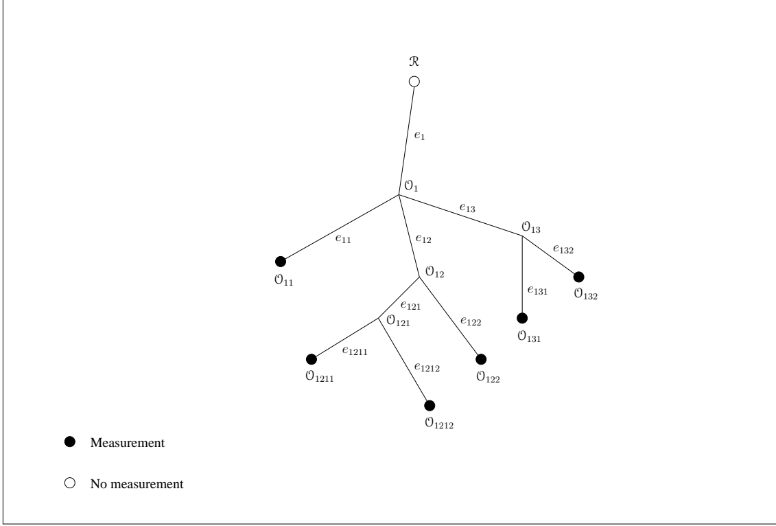
FIGURE 1. A tree with 10 edges.
