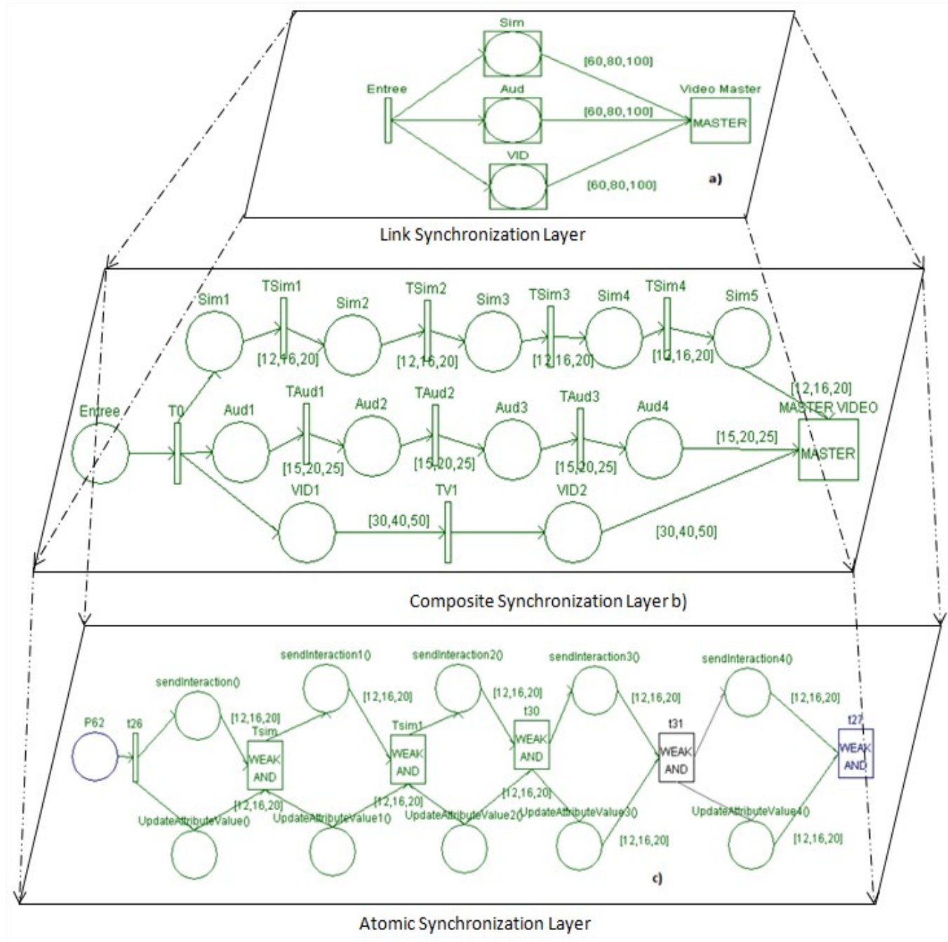
Figure 6. Distributed Multimedia Synchronization scheme over HLA-RTI. a) The link synchronization Layer, directly connected to the application b) the composite synchronization layer for the inter-stream synchronization Layer and c) the atomic synchronization layer which of the intra-flow synchronization
