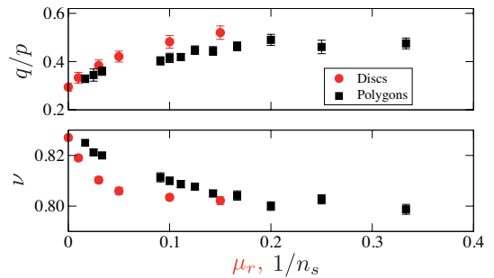
FIG. 1: (color online) Shear strength q/p (Up) and solid fraction \nu (Down) as functions of \mu_r for the disks and of 1/n_s for the polygons. Error bars indicate the standard deviation.
