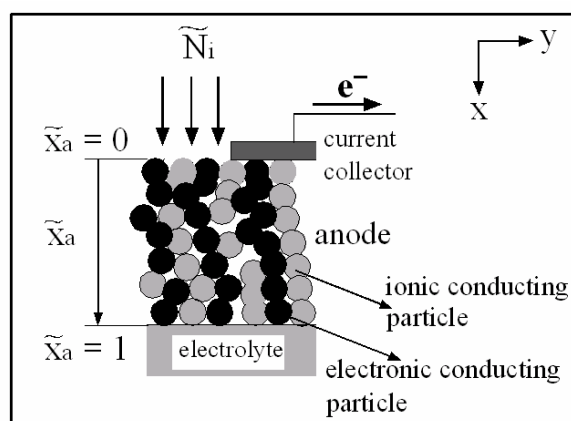
computational domain
