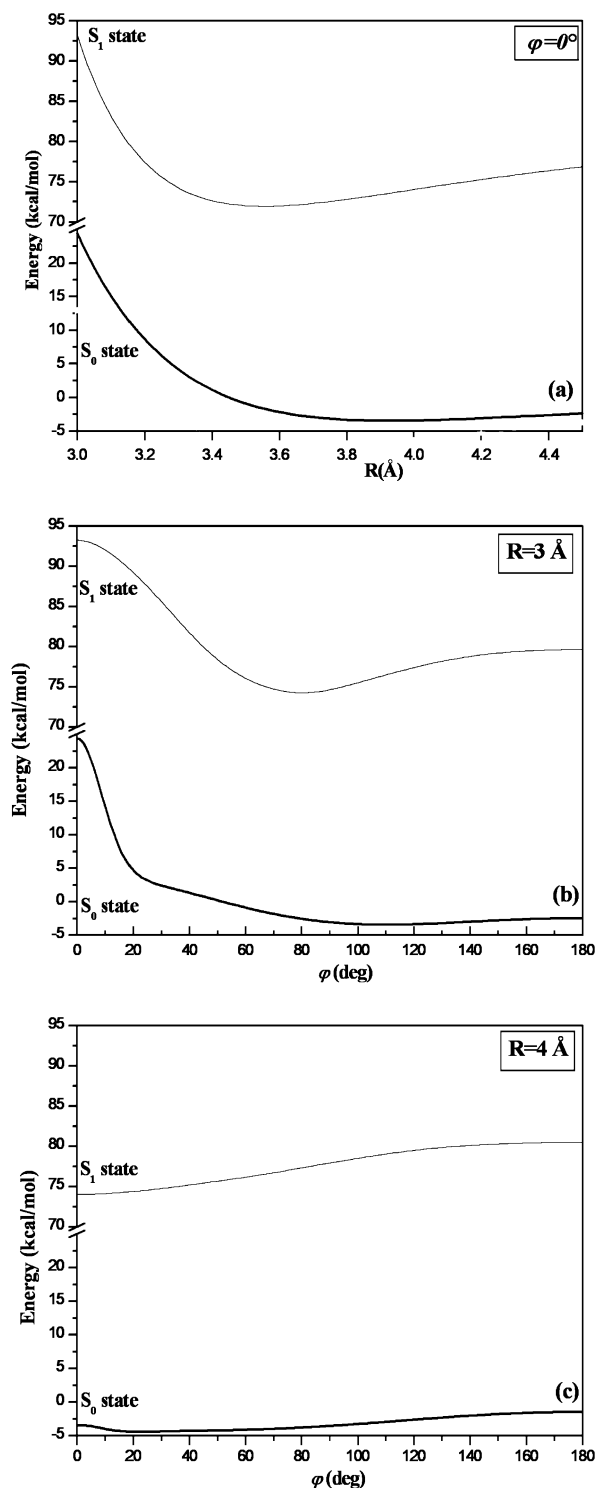
Figure 5. Interaction energy of the carbazole dimer in the S_0 and S_1 states: (a) sandwich-like configuration; (b and c) rotated structures about the pseudo X_1-X_2 bond (Figure 2) and for fixed intermolecular distance R .
