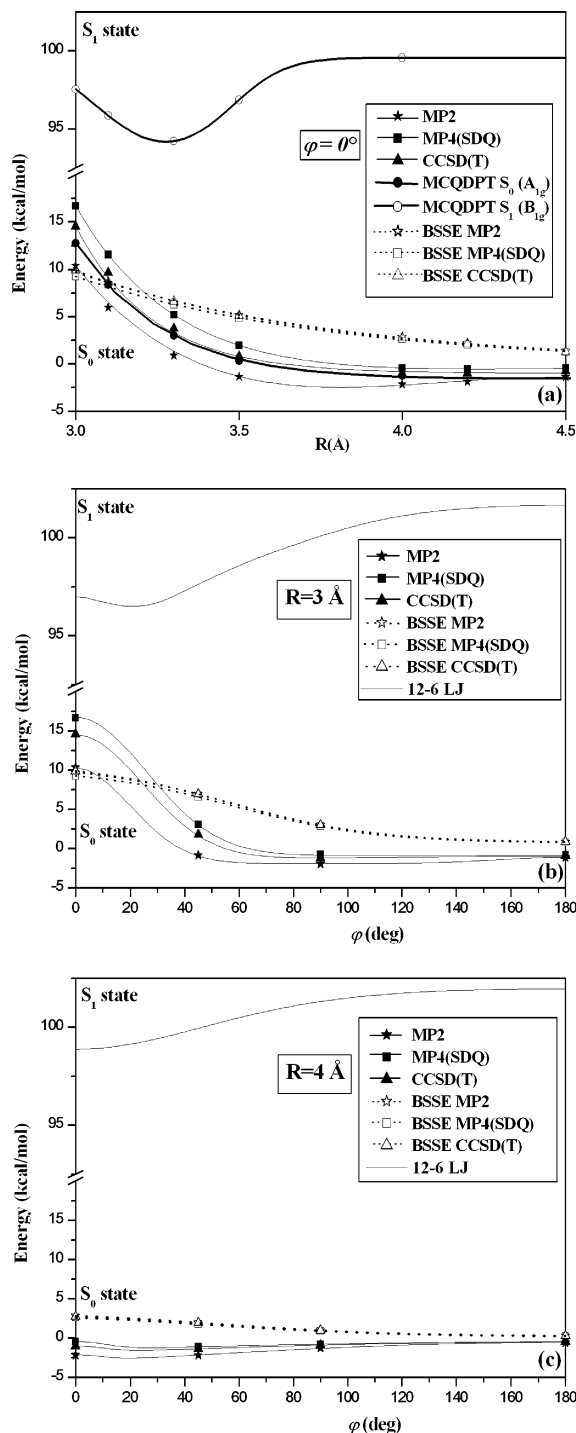
Figure 3. Ground-state and excited-state energy calculations with the modified cc-pvdz basis set for the benzene dimer in the (a) sandwich-like geometry ( \varphi = 0^\circ ) and (b and c) versus \varphi rotation about the ghost X_1-X_2 bond (Figure 2). Intermolecular distance is held fixed at (b) 3 Å or (c) 4 Å. The geometry of each benzene fragment is held fixed at the experimental geometry, and the energies are corrected for BSSE. The BSSE is indicated for the ground state (see text). Lines are only a guide to the eye. In addition, the 12-6 LJ potential ( S_1 state, Table 2) is also shown.
