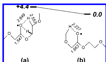
Figure 3. Minimum structures obtained for the alkoxy radical at the UB3P86/6-31++G(d,p) level of theory. Structure b is the less covalent, most stable geometry. Energies in kcal/mol; bond lengths in Å.
