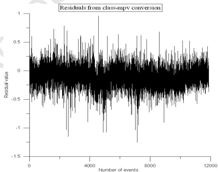
Fig. 3. Residuals from class to m_{pv} conversion.
