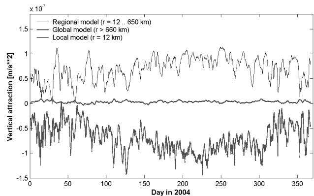
Figure 2: One year model time series of local (bottom), regional (top) and global (middle) fraction of atmospheric vertical attraction at Wettzell station. Local and regional series are shifted for better illustration.
