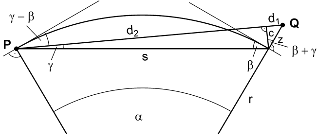
Figure 3: Geometrical relationships between observation site P and attracting mass point Q (see text).
