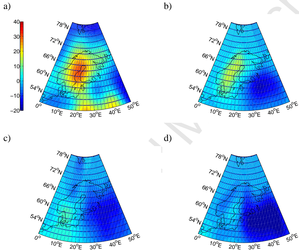
Fig. 4. Secular trends in Fennoscandia computed from GFZ GRACE monthly solution (a) as well as global hydrology models WGHM (b), LaDWorld (c) and GLDAS (d). Gaussian filter with 400 km radius was used. The time span is February 2003 to July 2007. Units are mm/year, in columns of equivalent water thickness.
