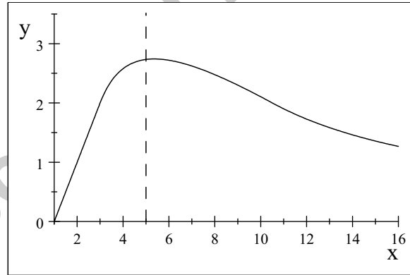
C5 Expected fitness for \gamma = 4 and \delta = 15
