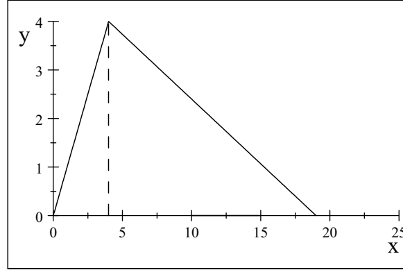
C4 Asymmetric fitness function with \gamma = 4, \delta = 15
