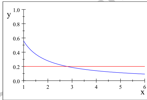
C2 Densities of group size (blue) and group size faced by a randomly chosen individual (red) for t = 5 .
