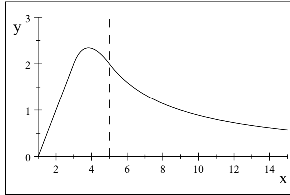
C3 Expected payoff for \gamma = 4
