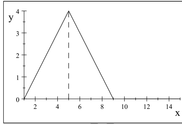
C1 Tent-shaped fitness function with \gamma = 4
