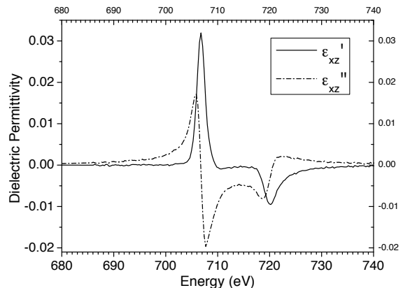
FIG. 4. Real and imaginary parts of the magnetic-dependent dielectric tensor elements of Fe atoms near the L_{3,2} edge.
