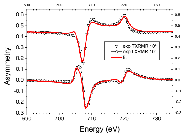
FIG. 8. Experimental (symbols) and calculated (solid line) asymmetry ratio vs energy for an incident angle of 10 degrees for (open circle) circular polarized light and longitudinal applied field (LXRMR) and, (triangles) for \pi -polarized light and transverse applied field (TXRMR) (with an offset of 0.45 for clarity).
