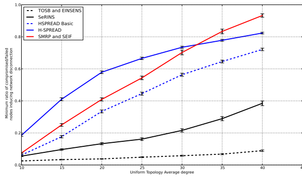
(a) Uniform topology
