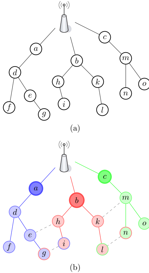
Figure 1: The concept of branch-aware flooding. (a) A topology obtained by a simple flooding protocol like the TinyOS beaconing protocol; (b) In a branch-aware protocol, the redundant reception of construction message can be exploited to discover new paths, without adding new messages. For instance, when node g broadcasts its message, the node i can discover an alternative path via the blue branch, since i already belongs to the red one. Nodes g and i are said to be cousin neighbors .
