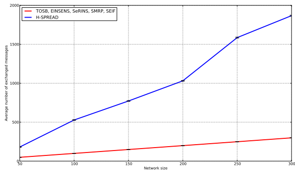
Figure 11: Number of exchanged messages during one round
