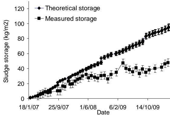
Figure 5. Evolution of biosolid accumulation at 30 kgSS/m 2 /y.
