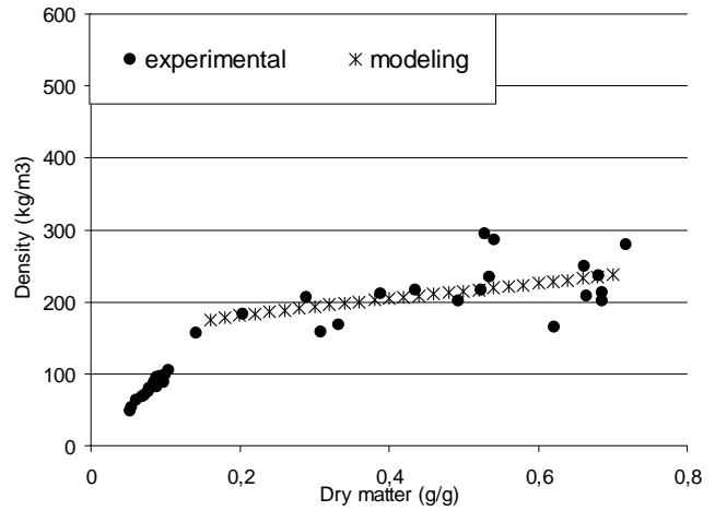
Figure 4. Apparent solid density vs DM.
