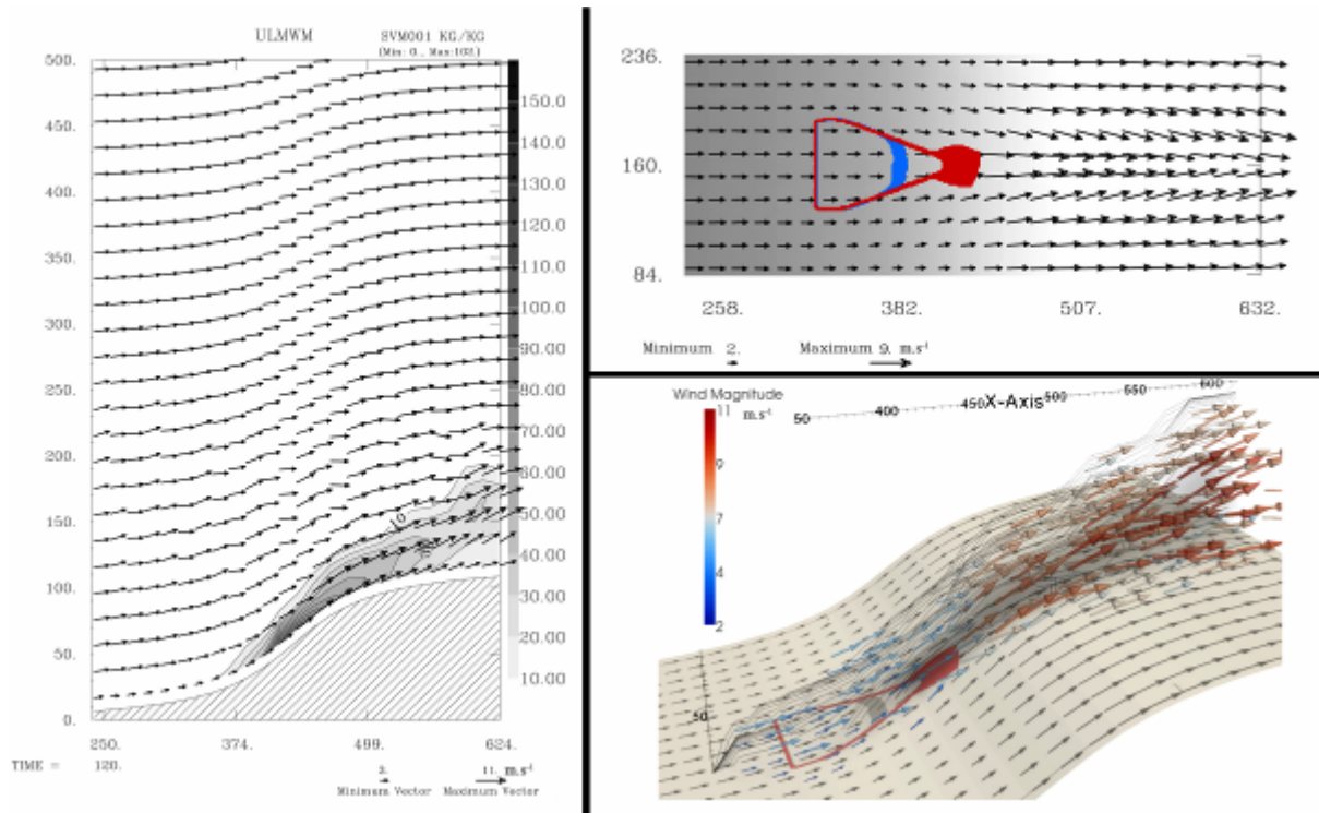
Fig. 5. HILL (a) Horizontal section (x/y) at Z=10\text{m} , fire lines after 120 seconds for the coupled (red) and non-coupled (grey) simulations. Arrows denote the wind vectors at ground level for the coupled-case. (b) Cross section (x/z) of the coupled case at Y=160\text{m} , shading represents concentration of the injected passive tracer. (c) 3d wind field and passive tracer concentration isocontours.
