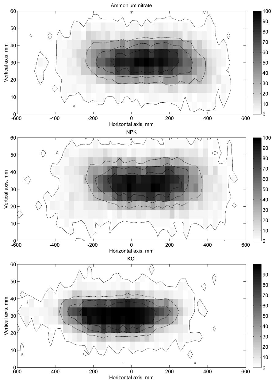
Fig. 4. Two-dimensional distribution of the mass flow. The grey scale corresponds to the fraction intercepted by the block (in percent) relative to the maximum intercepted amount by a sampled block (5 × 25 mm).
