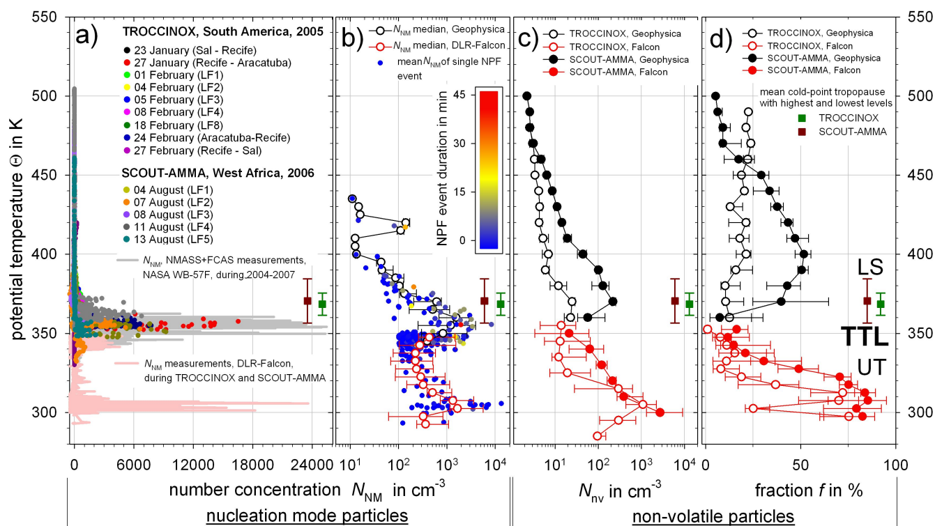
Fig. 3. (a) Colored circles: concentrations of nucleation mode particles, N_{NM} , in the size range 6\text{ nm} < d_p < 15\text{ nm} (COPAS) of 9 tropical flights of the M-55 “Geophysica” during TROCCINOX (4 transfer and 5 local flights) and of 5 local flights during SCOUT-AMMA. Rose colored: N_{NM} ( 4\text{ nm} < d_p < 15\text{ nm} ) from CPC measurements on the DLR Falcon-20 throughout both campaigns ( \Theta < 350\text{ K} ). Grey colored: N_{NM} ( 5.3\text{ nm} < d_p < 15\text{ nm} ) resulting from 4 yr of measurements with the NMASS system (on the NASA WB-57F). (b) Solid lines: median vertical distribution of N_{NM} with 25th and 75th percentiles from COPAS measurements (black) and DLR Falcon-20 CPC measurements (red). Circles: averaged N_{NM} of single NPF events, color-coded according to the observed event duration. (c) Median vertical profile with 25th and 75th percentiles of the number concentration ( N_{nv} ) of non-volatile particles with d_p > 1.0\text{ nm} . (d) Median vertical profile with 25th and 75th percentiles of the fraction f = N_{nv}/N_6 of non-volatile particles (black: COPAS measurements; red: DLR Falcon-20 CPC data). Squares with vertical bars: mean cold point tropopause (green: TROCCINOX; dark-red: SCOUT-AMMA) with bars denoting the highest and lowest encountered tropopause heights.
