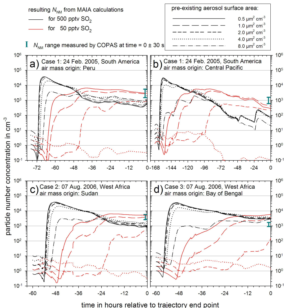
Fig. 7. Model calculation of particle number concentration, N_{NM} , as measure for the strength of NPF caused by neutral and ion-induced binary aerosol nucleation of H_2SO_4 - H_2O droplets computed by the kinetic aerosol model MAIA (using FLEXTRA trajectories shown in Fig. 6). See text and Table 2 for details and model input parameters. Lines: N_{NM} produced by nucleation of H_2SO_4 , oxidized from SO_2 , and H_2O as function of time before the air parcel was sampled by the aircraft (at time = 0) and as a function of pre-existing aerosol surface area. Black lines: assuming a pre-existing SO_2 mixing ratio of 500 pptv. Red lines: for 50 pptv initial SO_2 . Green vertical bars: COPAS measurement of N_{NM} at time = 0 (slightly displaced from t = 0 for clarity).
