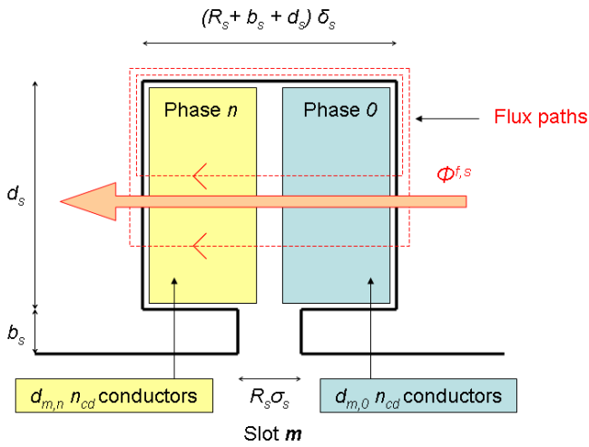
Fig. 9. Assumptions for the flux paths inside the iron to estimate the leakage inductance of a slot
