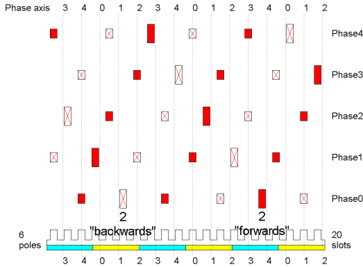
Fig. 4. Example of an irregular balanced fractional winding for 5-phase machine with 6 poles and 20 slots ( s_{pp} = 2/3 )
