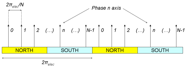
Fig. 1. Representation of a balanced multi-phase winding distribution ( \pi_{elec} = \frac{\pi}{p} , p the pole pair number, p = 2 in the figure)
