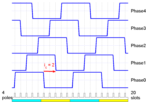
Fig. 6. Winding function for the winding distribution described in figure 2
