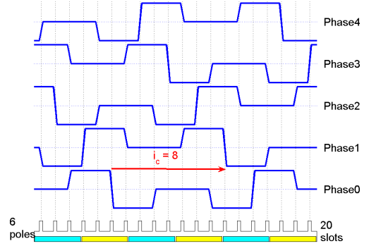
Fig. 7. Winding function for the fractional winding distribution described in figure 4
