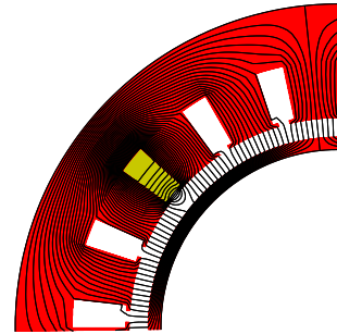
Fig. 10. Flux path for M5-A machine ( s_{pp} = 1 ) where a single phase is supplied
