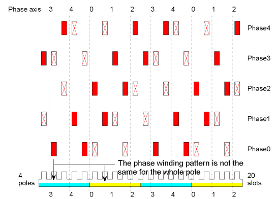
Fig. 3. Example of an irregular integral-slot balanced winding with holes: case of a 5-phase machine with 4 poles and 20 slots ( s_{pp} = 1 )
