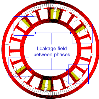
Fig. 11. Flux path for M5-B machine ( s_{pp} = 1 ) where a single phase is supplied
