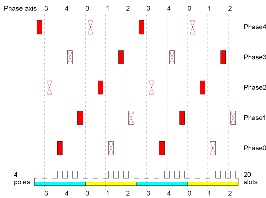
Fig. 2. Example of a regular integral-slot balanced winding : case of a 5-phase machine with 4 poles and 20 slots ( s_{pp} = 1 ), the winding pattern is the same for each pole and each phase
