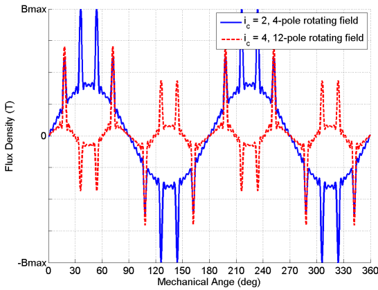
Fig. 5. Comparison of the air gap flux density obtained with i_c = 2 and i_c = 4 for a 5-phase machine (winding of figure 2 where (p, N_s) = (2, 20) )
