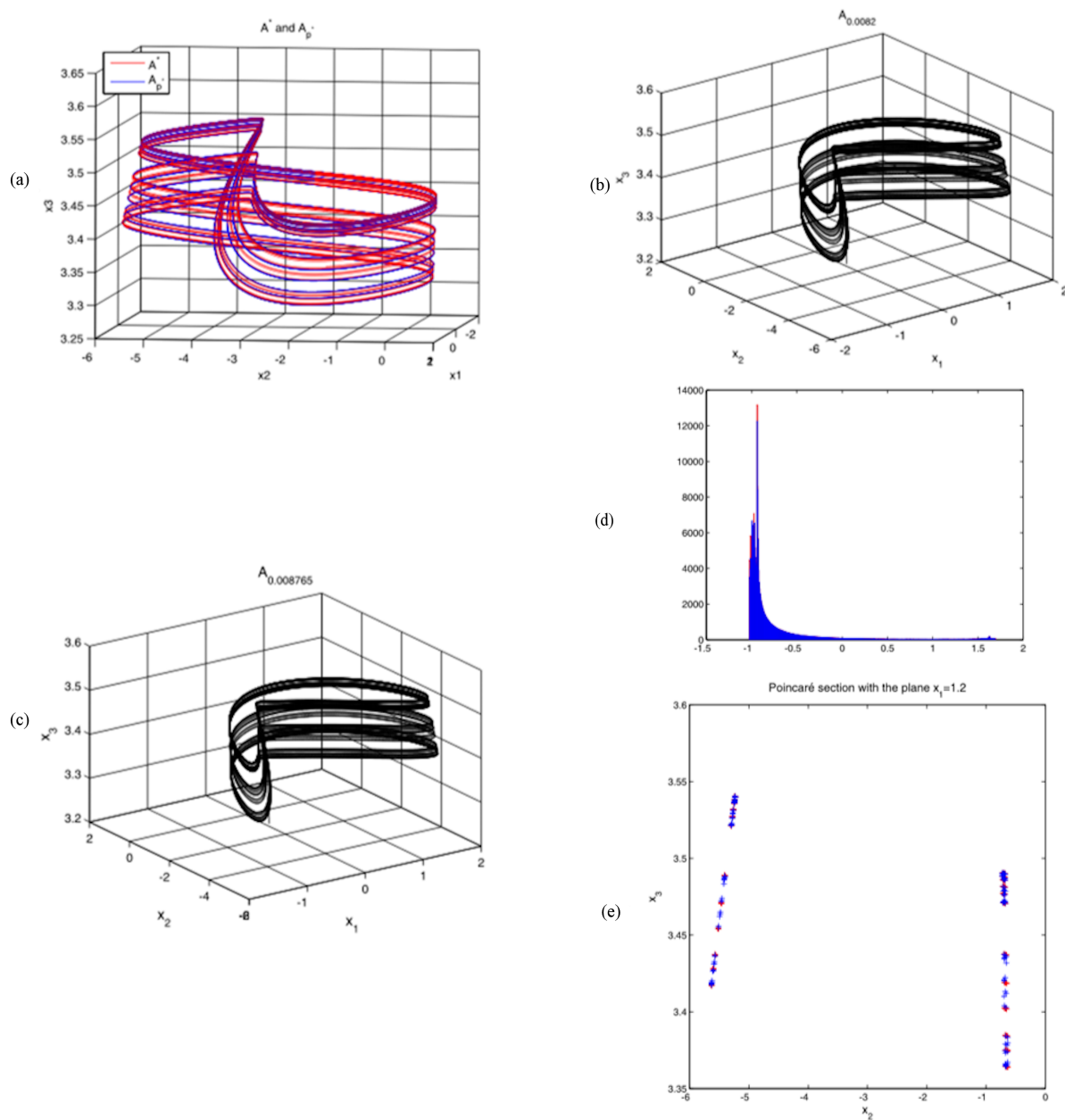
Fig. 5 AS algorithm for N = 2 and \mathcal{P}_N = \{0.0082, 0.008765\} and m_1 = m_2 = 1 ; a) A^* and A_{p^*} , with p^* = 0.0084825 , superimposed; b) A_{0.0082} ; c) A_{0.008765} ; d) Superimposed histograms of A^* and A_{p^*} ; e) Superimposed Poincaré sections of A^* and A_{p^*} for x_1 = 1.2 .
