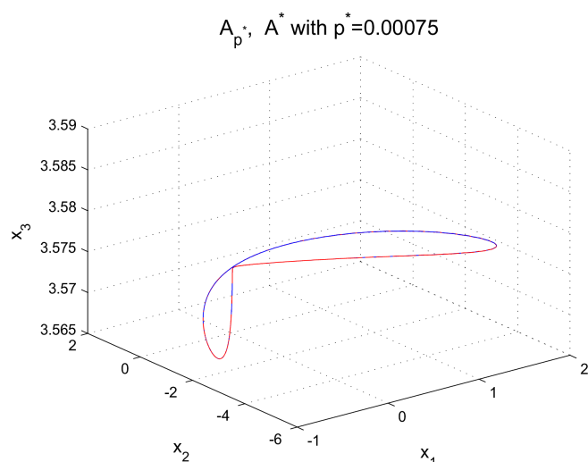
Fig. 4 AS algorithm for N = 10 , p_i = 0.0002 + i \times 0.0001 and m_i = 1 , for i = 1, 2, \dots, 10 ; A^* and A_{p^*} , with p^* = 0.00075 , are superimposed.
