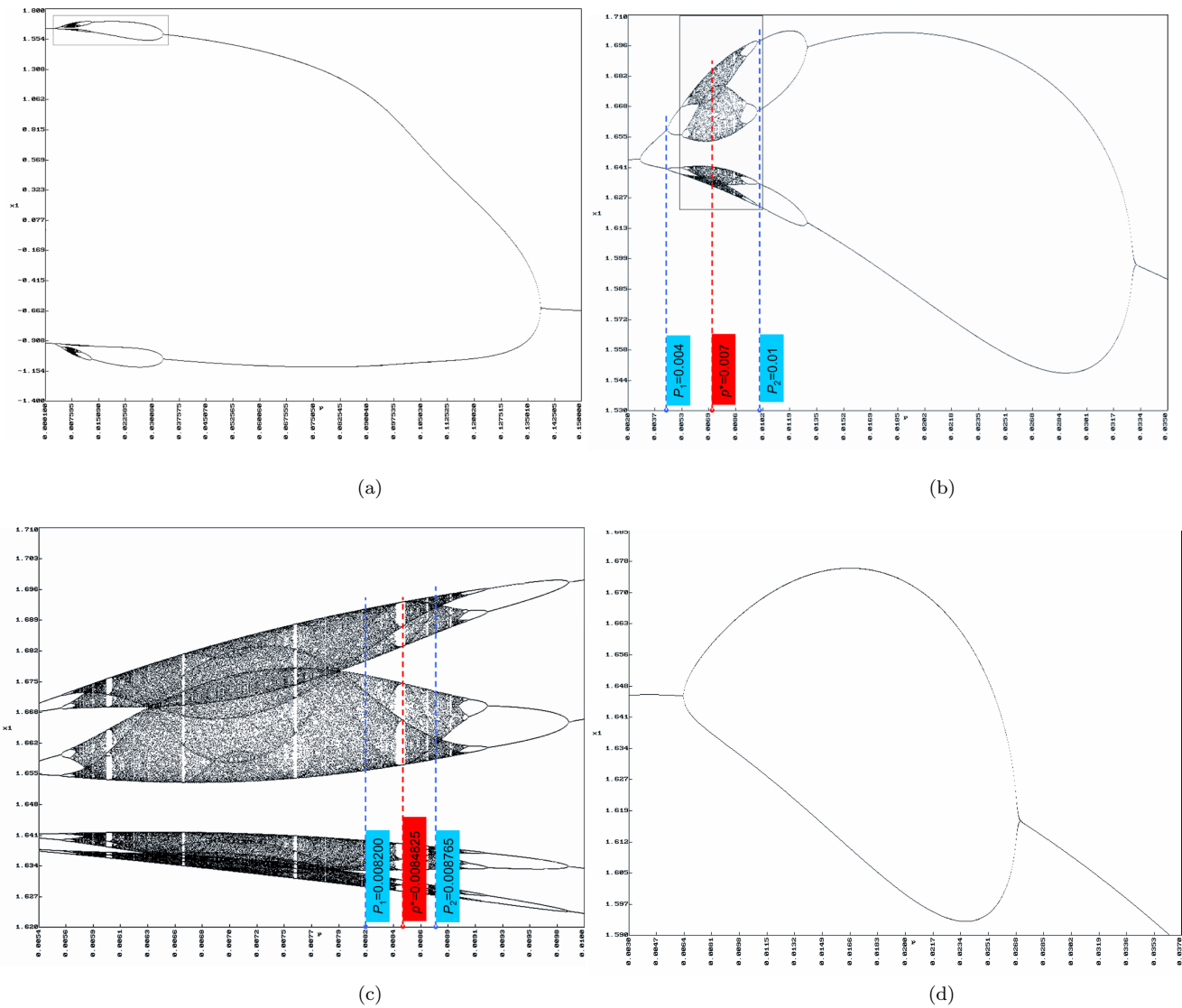
Fig. 1 (a) Bifurcation diagram: x_1 vs p with I = 3.4 . (b) Detail of Fig. 1a. (c) Consecutive detail of Fig. 1b. (d) Bifurcation diagram: x_1 vs p with I = 3.5 .
