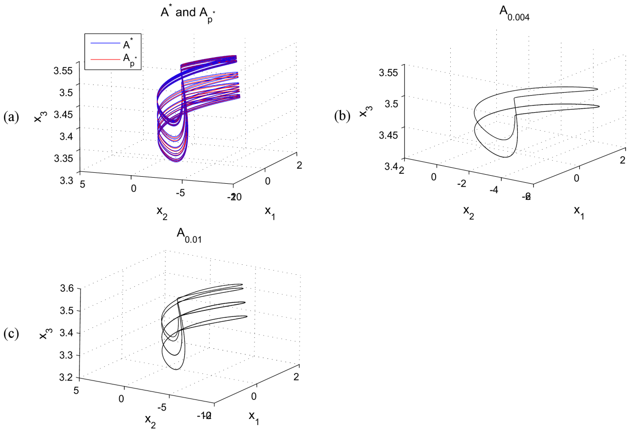
Fig. 3 AS algorithm with scheme [1p_1, 1p_2] with p_1 = 0.004 and p_2 = 0.01 ; a) The synthesized and averaged attractors A^* and A_{p^*} respectively, superimposed for p^* = 0.007 ; b) Attractor A_{0.004} ; c) Attractor A_{0.01} .
