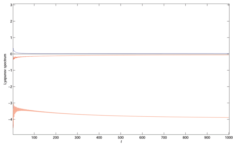
Fig. 6 Temporal evolution of Lyapunov exponents for p = 0.0084825 .
