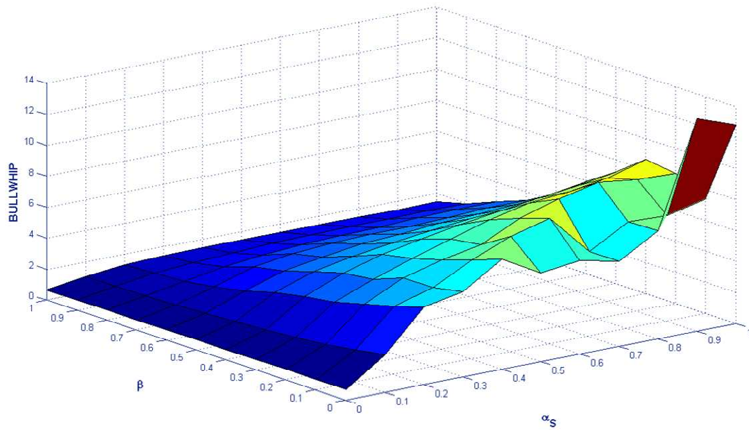
Figure 3 – Surface of the bullwhip suffered by retailer in the case of multi-stage model and for customer demand given by scenario 3 plotted with respect to the \alpha_s and \beta parameters.
