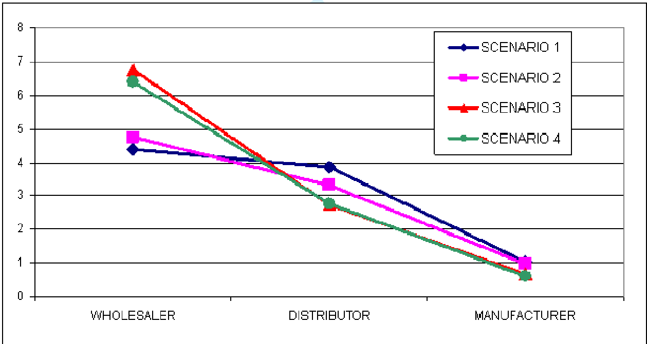
Figure 6 – Average values of inventory oscillations with respect to supply chain sector, single-stage model.
