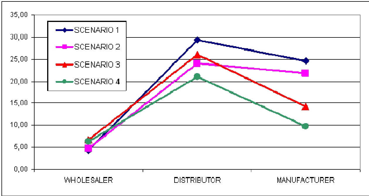
Figure 7 – Average values of inventory oscillations suffered by the actors in a multi-stage model.
