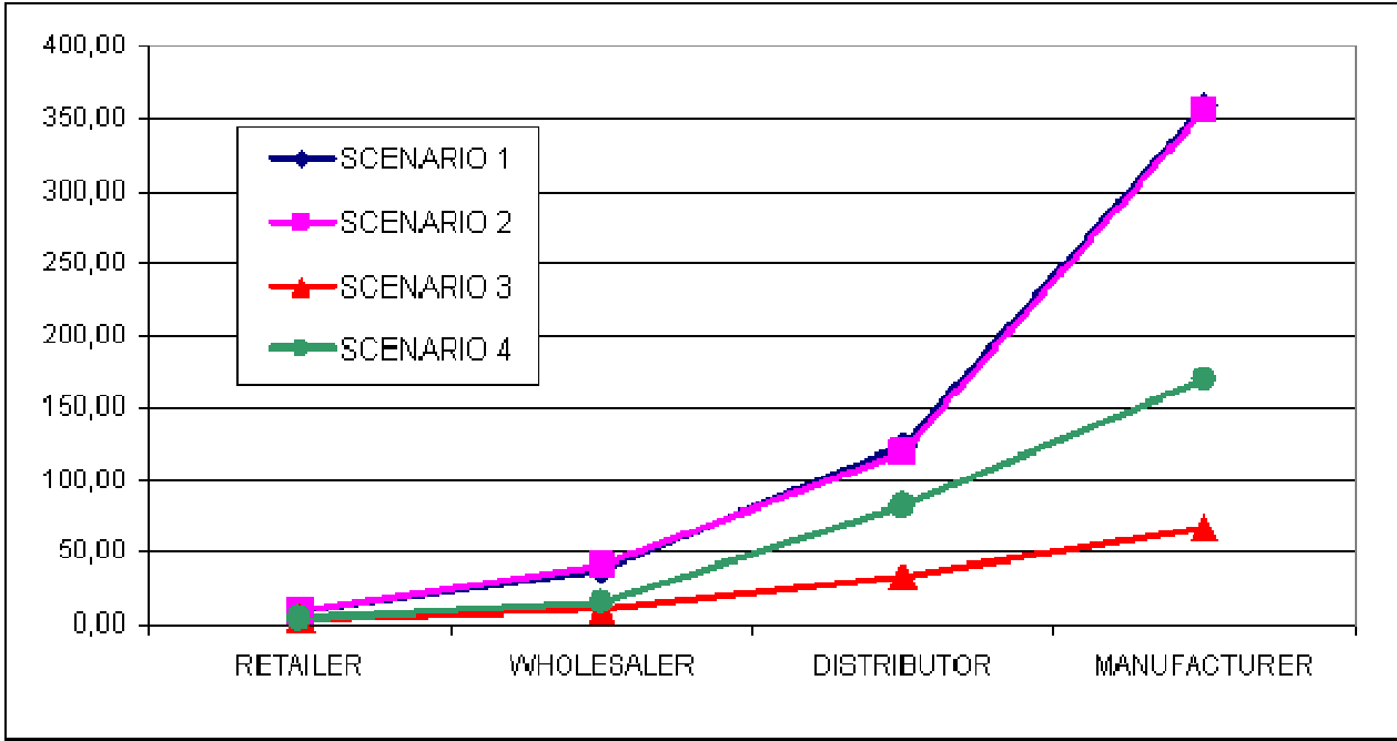
Figure 5 – Increasing of mean Bullwhip values going upstream in the supply chain in the case of the multi-stage model.
