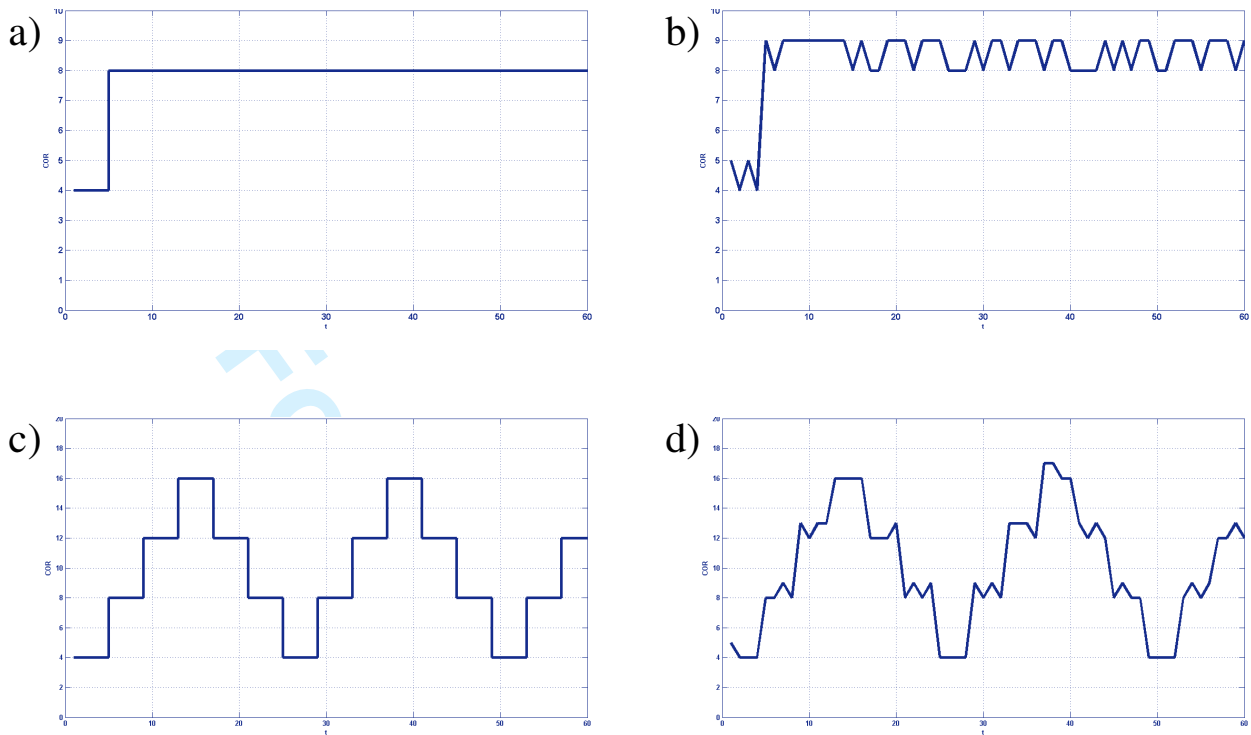
Figure 1 – Types of final customer demand (COR) analyzed: a) step; b) step with noise with variance 1; c) cyclic; d) cyclic with noise with variance 1.
