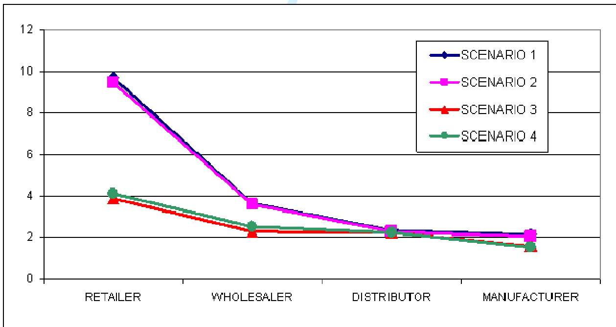
Figure 4 – Decreasing of mean bullwhip values going upstream in the supply chain in the case of the single-stage model.
