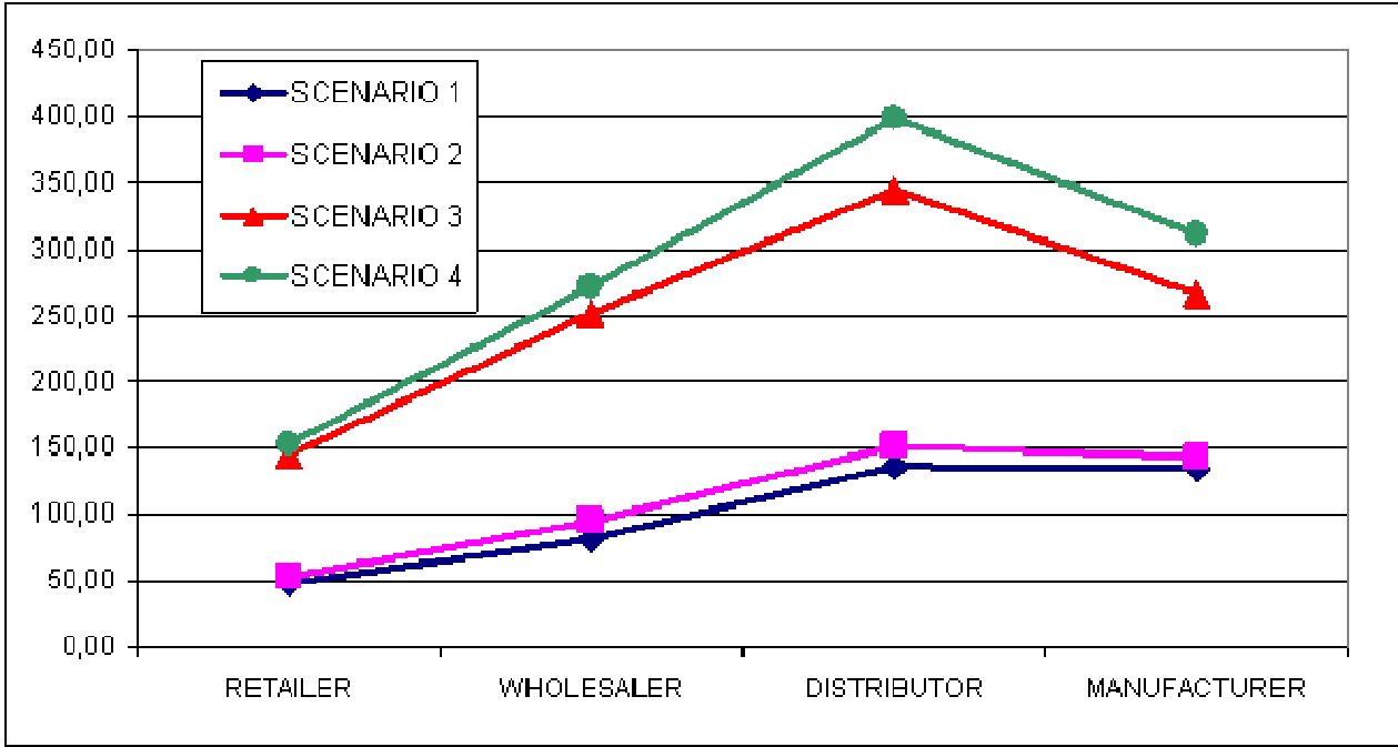
Figure 9 – Average inventory maximum oscillations with respect to supply chain sector.
