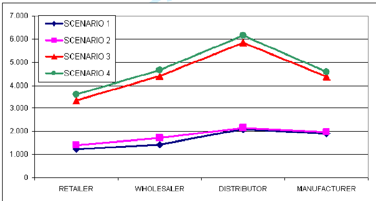
Figure 8 – Average management costs of the inventory for each level.
