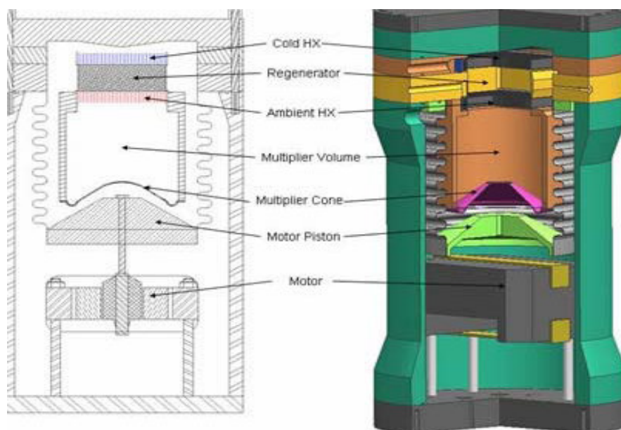
Figure 8. Travelling wave thermoacoustic device (Ben & Jerry ice-cream cabinet [48])
