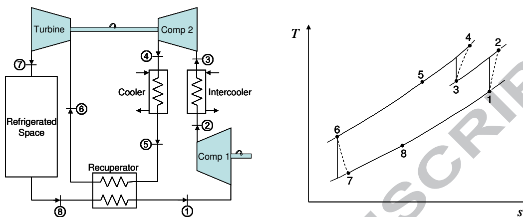
Figure 3. Air cycle with regenerative heat exchange and two-stage compression with intercooling.
