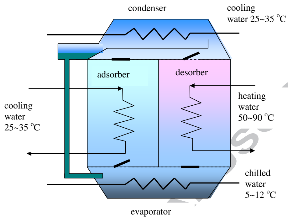
Figure 1. Schematic diagram of adsorption refrigeration system
