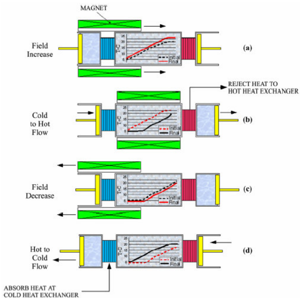
Figure 9. Active magnetic regeneration cycle (from Russek and Zimm [50])
