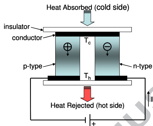
Figure 6. Thermoelectric cooling (or Peltier) couple
