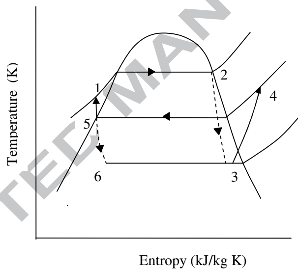
Figure 2. Schematic and T-s diagram of ejector refrigeration system
