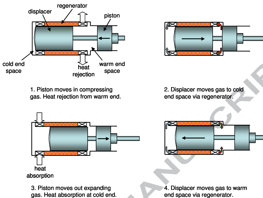
Figure 5. Piston and displacer movements during a Stirling refrigeration cycle.
