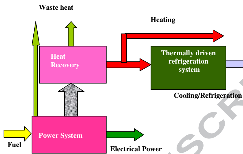
Figure 4. Schematic of a trigeneration system
