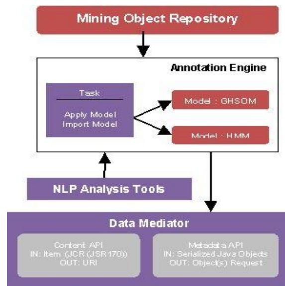
Figure 5.16: Annotation Engine
