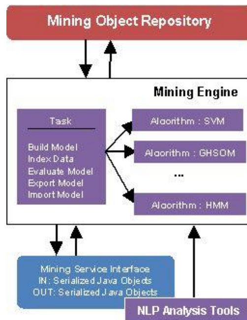
Figure 5.15: Mining Engine
