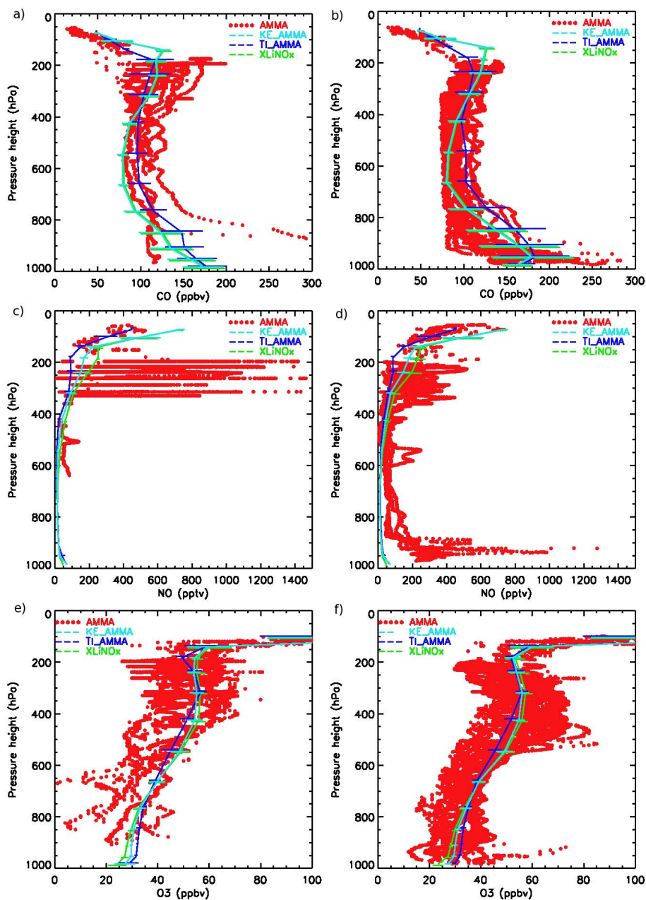
Fig. 3. Vertical CO (a, b), NO (c, d) and O 3 (e, f) profiles observed (red dots) during the AMMA campaign in August 2006 and simulated by KE_AMMA, TL_AMMA and XLiNOx. Observations and model results were divided into flights recently impacted by convection (left) and not impacted by recent deep convection (right). See text for details. The horizontal lines indicate the standard deviation in the model results.
