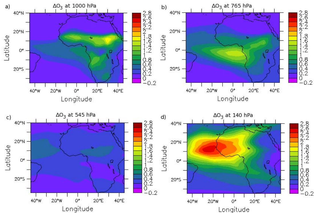
Fig. 8. KE_AMMA - BIO_red O 3 differences ( \Delta\text{O}_3 ) in ppbv at 1000 hPa (a), 765 hPa (b), 545 hPa (c) and 140 hPa (d).
