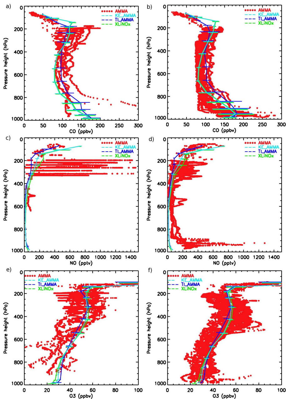
Fig. 3. Vertical CO (a, b), NO (c, d) and O 3 (e, f) profiles observed (red dots) during the AMMA campaign in August 2006 and simulated by KE_AMMA, TI_AMMA and XLiNOx. Observations and model results were divided into flights recently impacted by convection (left) and not impacted by recent deep convection (right). See text for details. The horizontal lines indicate the standard deviation in the model results.
