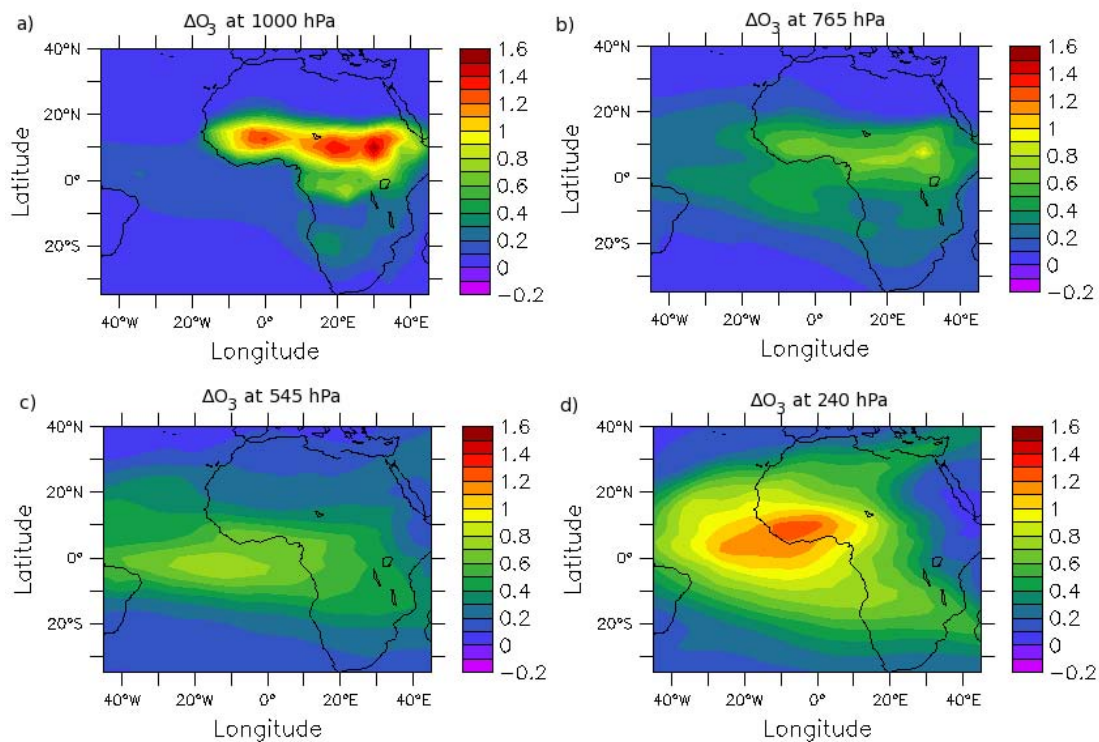
Fig. 7. KE_AMMA-SNOx_red O 3 differences ( \Delta\text{O}_3 ) in ppbv at 1000 hPa (a), 765 hPa (b), 545 hPa (c) and 240 hPa (d).
