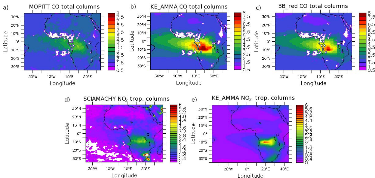
Fig. 5. Total columns of CO ( 10^{18} molec \text{cm}^{-2} ) and tropospheric columns of NO 2 ( 10^{15} molec \text{cm}^{-2} ) observed by MOPITT (a) and SCIAMACHY (d) respectively and corresponding KE_AMMA and BB_red simulations (b, c, e) averaged for August 2006.
