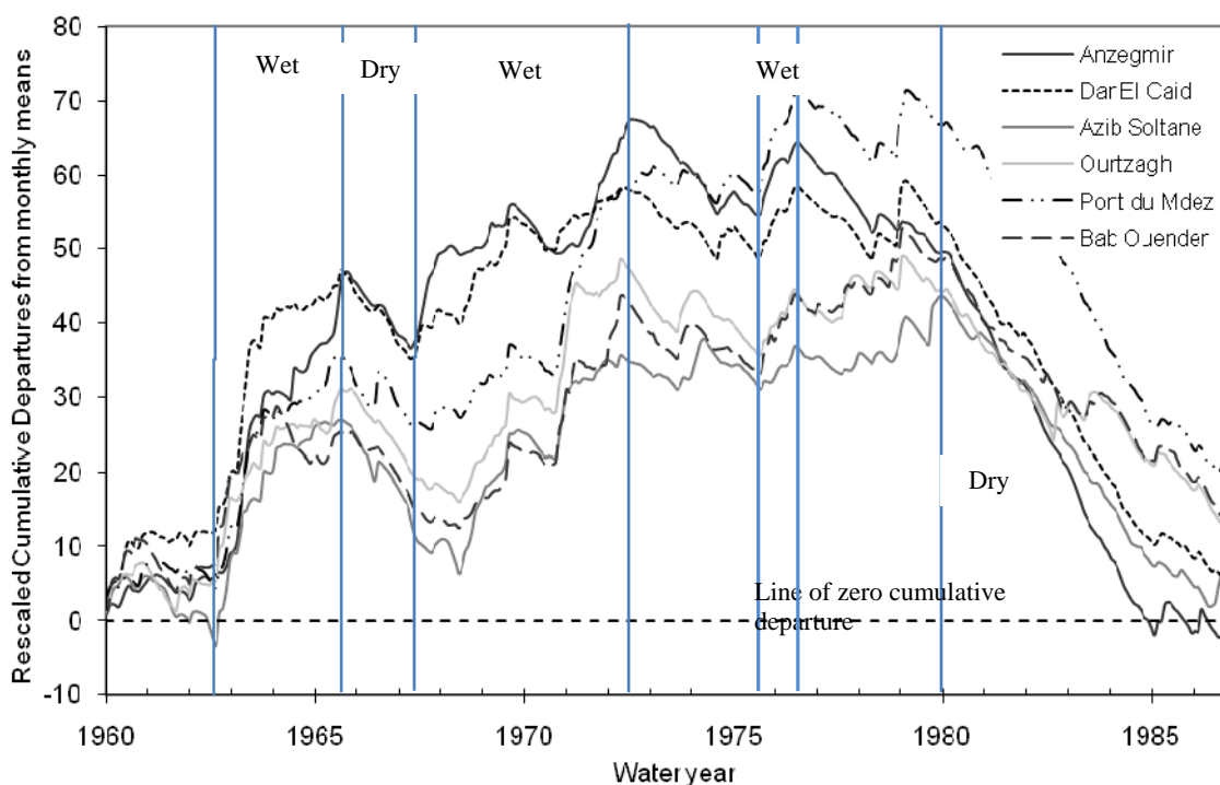
Figure 2: Rescaled Cumulative Departures of monthly mean streamflow, 1960-1987
