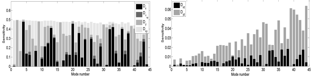
Figure 3: Sensitivities of the modal frequencies to the real parts of the rigidities given by Eqs. 8. Each column is the sum of the sensitivities to D_x , D_{v,xy} , D_y , and D_{xy} (left frame) and to D_{xz} and D_{yz} (right frame). The total may exceed 0.5 since some sensitivities are negative. the different involved parameters.
