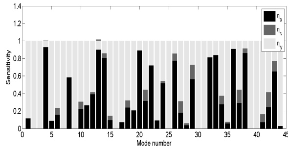
Figure 4: Sensitivities of the modal dampings to the dissipative parameters of the fictitious material of the equivalent homogenised plate \eta_x^H , \eta_{v,xy}^H , \eta_y^H , and \eta_{xy}^H .
