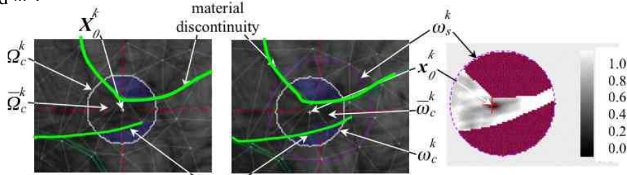
FIG. 2 – WDP method : (a) zoom of the reference picture S_0 showing the correlation domain \Omega_c^k of radius r_c and center \underline{X}_0^k and the effective correlation domain \bar{\Omega}_c^k delimited by a crack and a material discontinuity, (b) zoom of the deformed picture S_n ( n = 4 ) showing the correlation domain \omega_c^k of center \underline{x}_0^k located in the search domain \omega_s^k of radius r_s and centered at \underline{x}_0^k ; \bar{\omega}_c^k is the effective correlation domain. (c) Correlation coefficient field in \omega_s^k .
